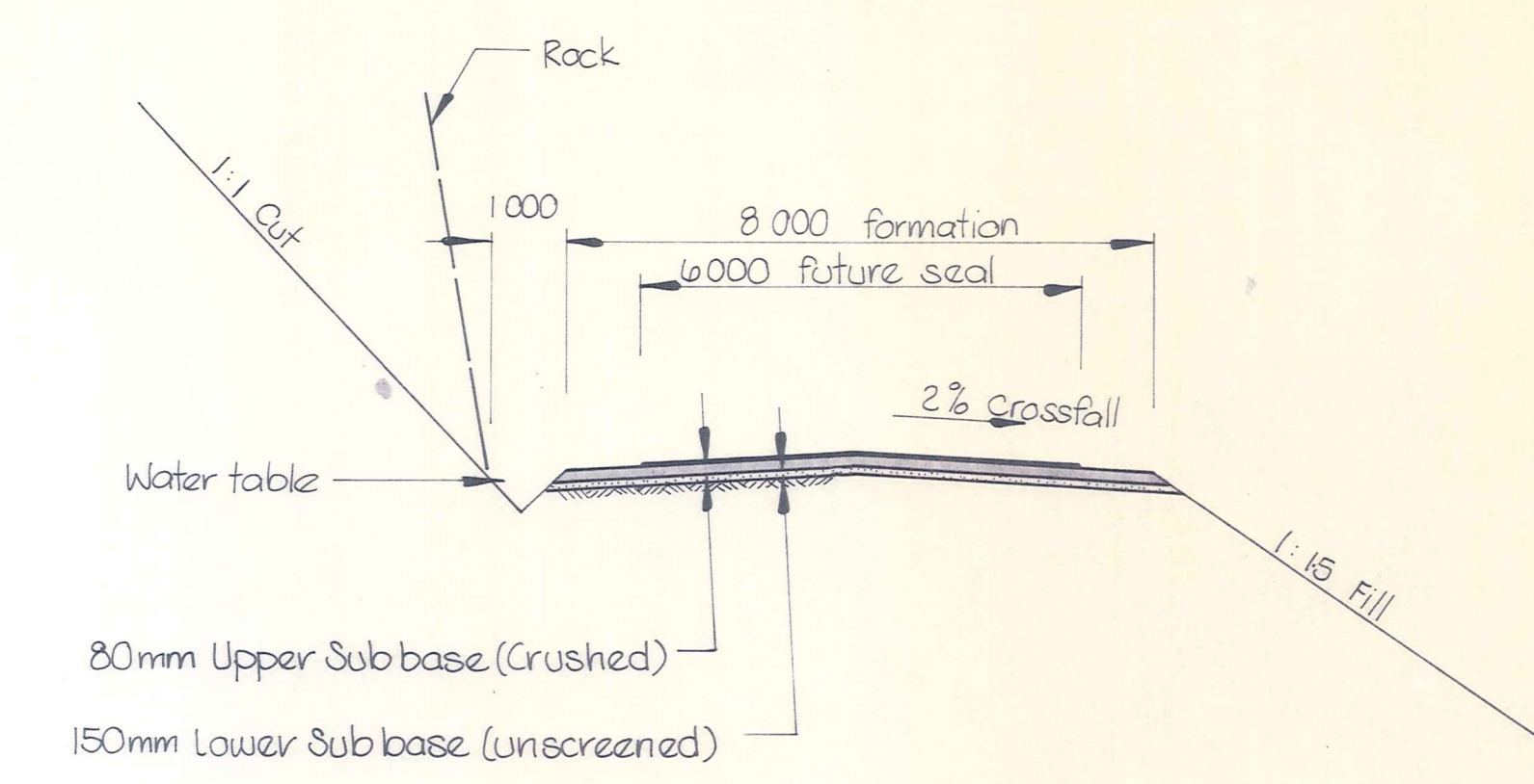
TYPICAL ROADING CROSS SECTION 1:100
