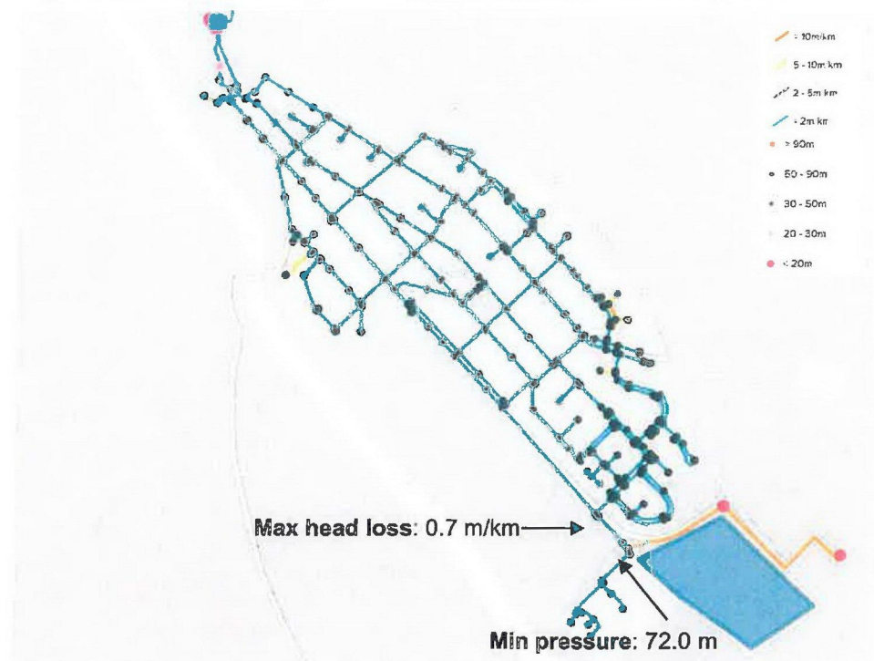
Figure 4 - Existing Peak Day - After Mutton Town Road Development
