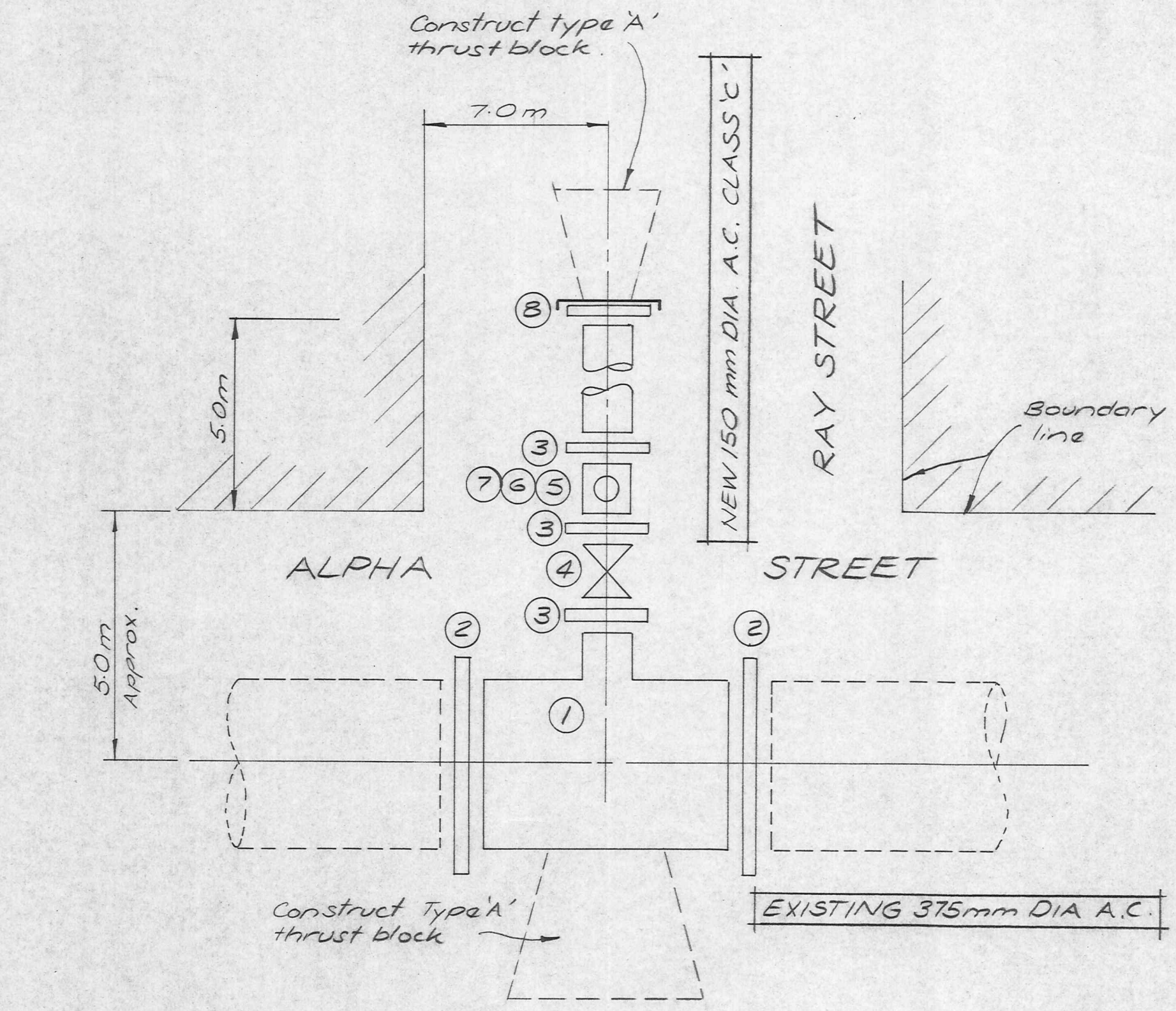
WATERMAIN DIAGRAM INTERSECTION OF ALPHA ST. AND RAY ST. N.T.S.
