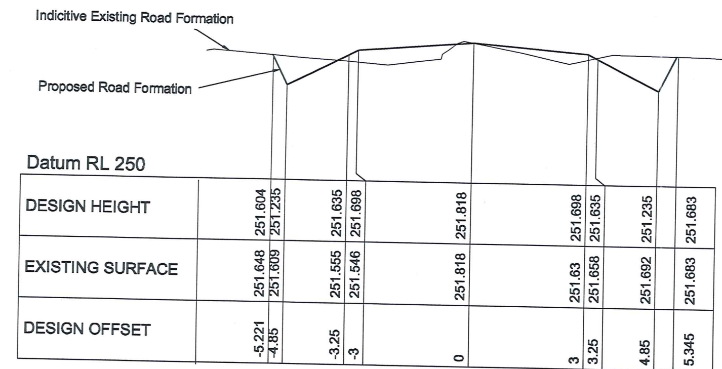
CHAINAGE 400 HORIZONTAL 1:100 VERTICAL 1:50
