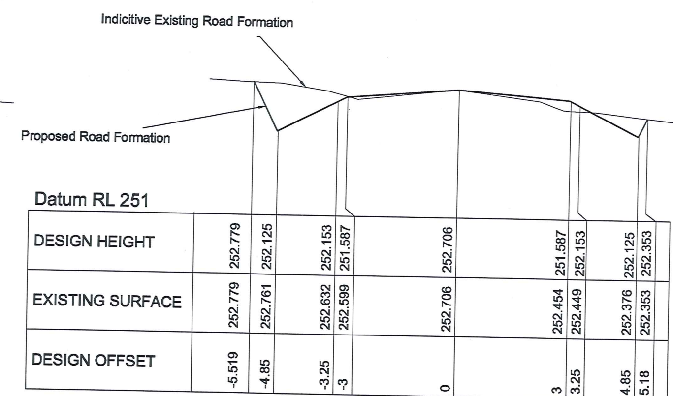
CHAINAGE 500 HORIZONTAL 1:100 VERTICAL 1:50
