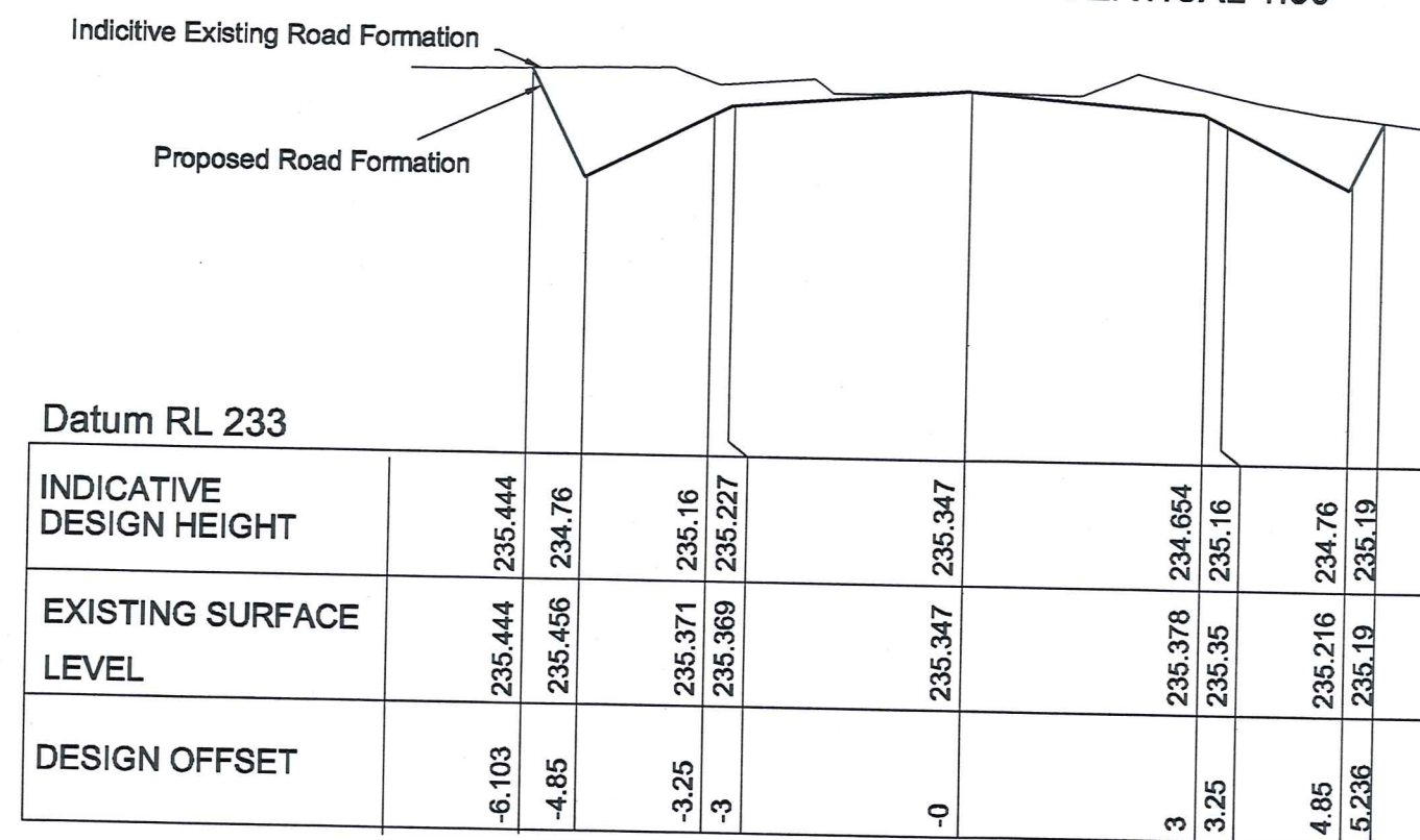
CHAINAGE 0. HORIZONTAL 1:100 VERTICAL 1:50
