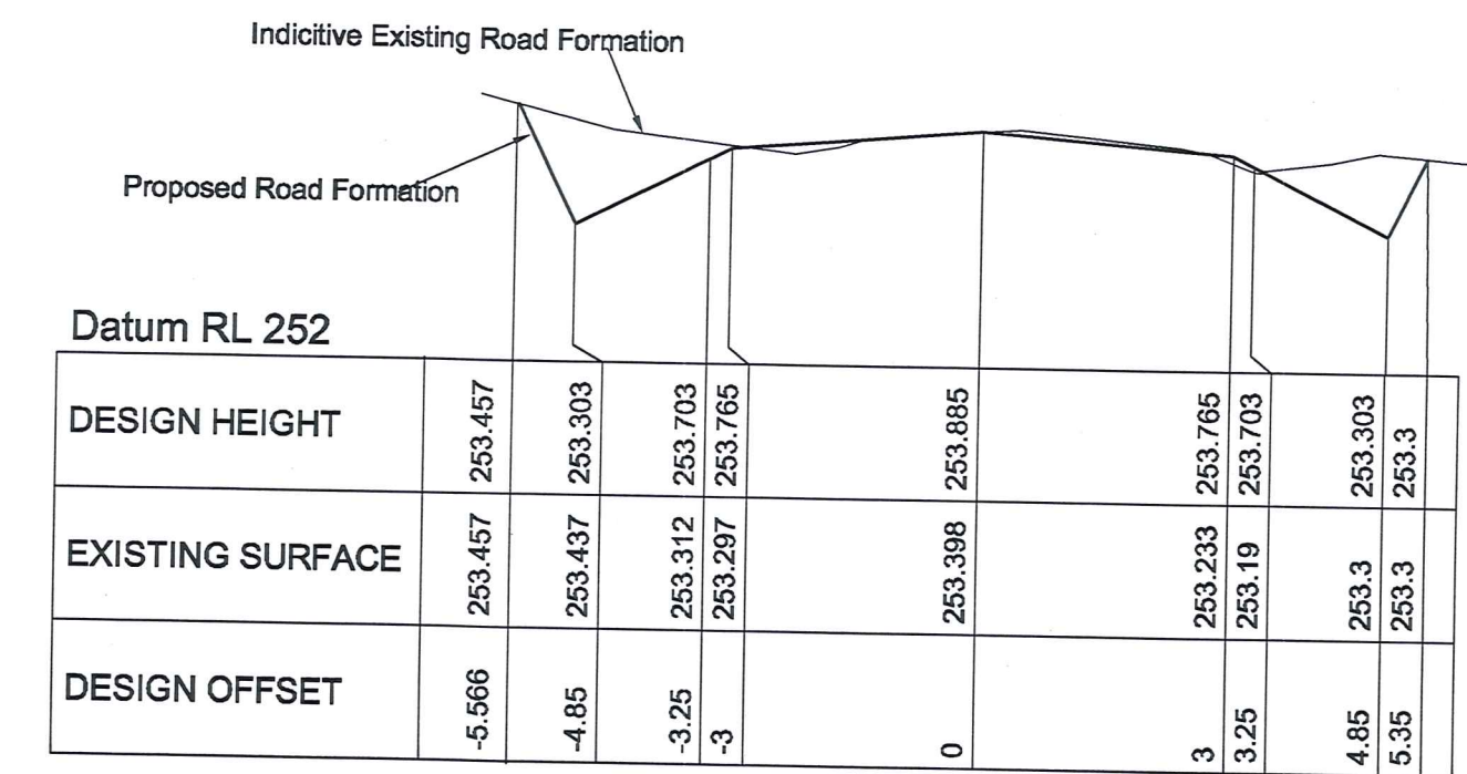
CHAINAGE 600 HORIZONTAL 1:100 VERTICAL 1:50
