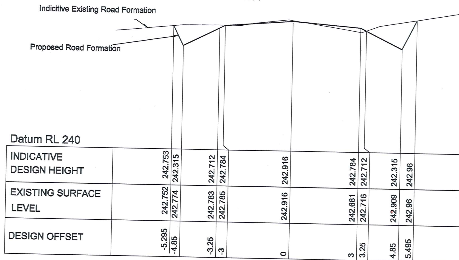
CHAINAGE 100. HORIZONTAL 1:100 VERTICAL 1:50
