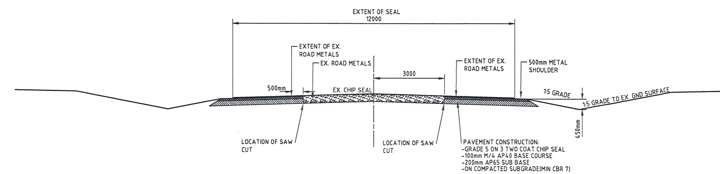
TYPICAL CROSS SECTION OF SPRINGVALE RD AND McARTHUR RD INTERSECTION WIDENING SCALE 1:100
