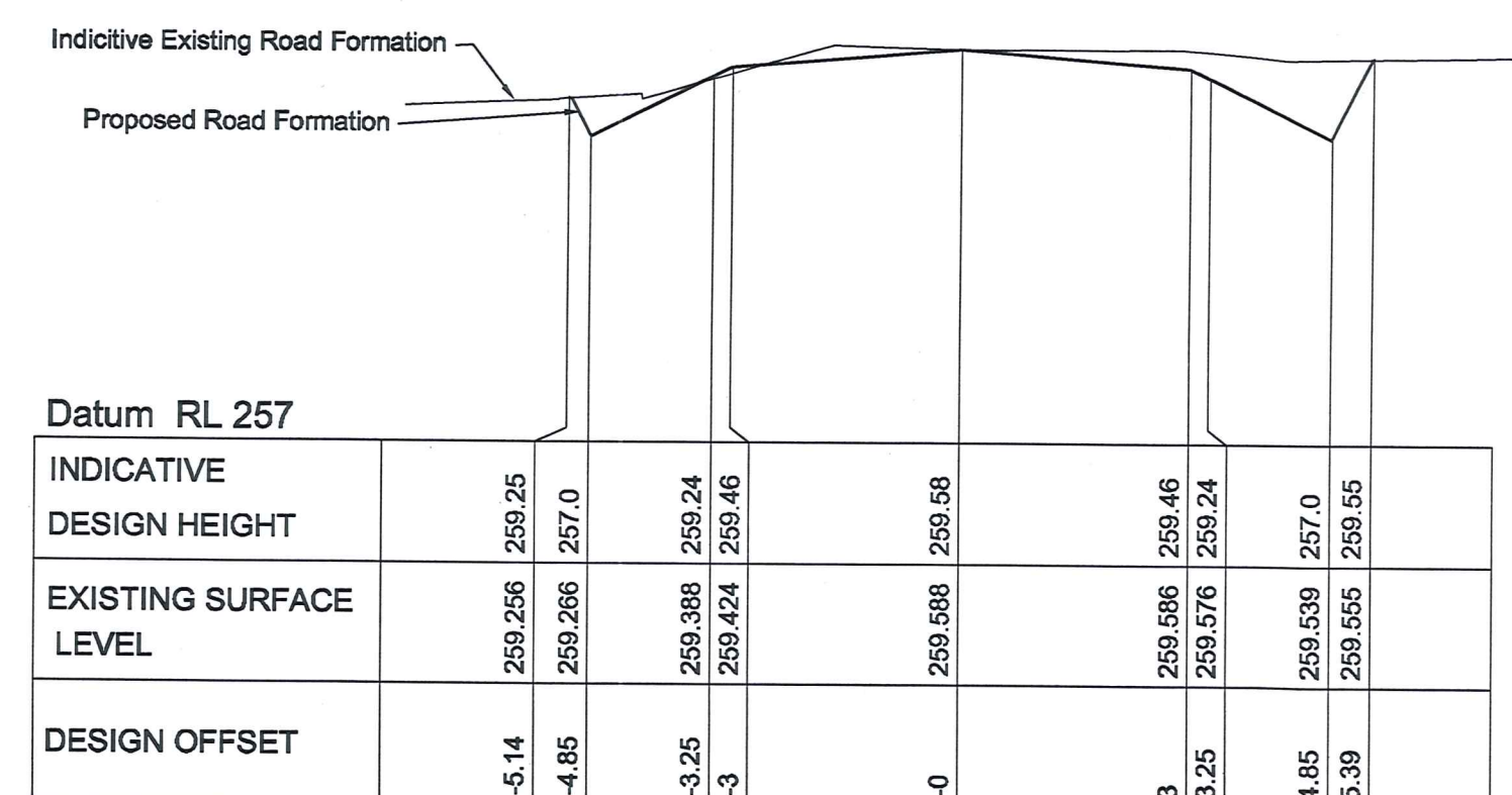
CHAINAGE 900 HORIZONTAL 1:100 VERTICAL 1:50
