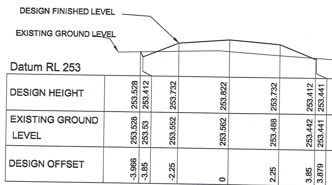
CHAINAGE 0.
