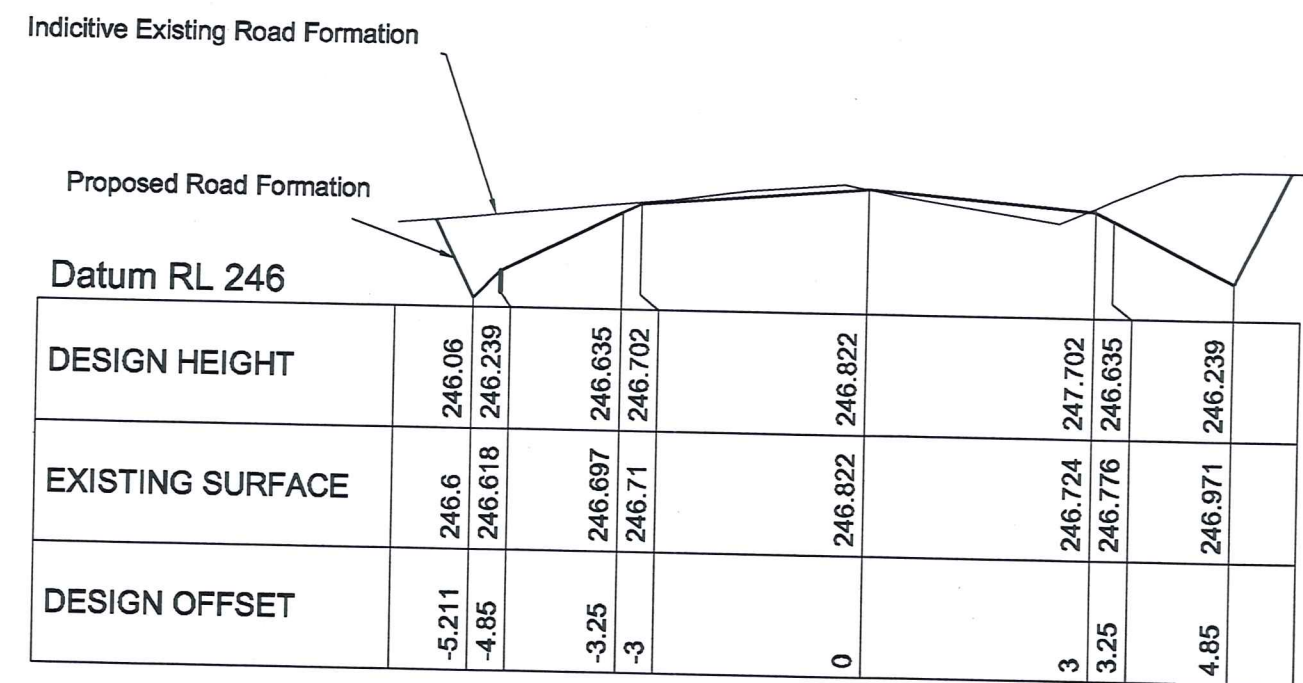
CHAINAGE 200. HORIZONTAL 1:100 VERTICAL 1:50
