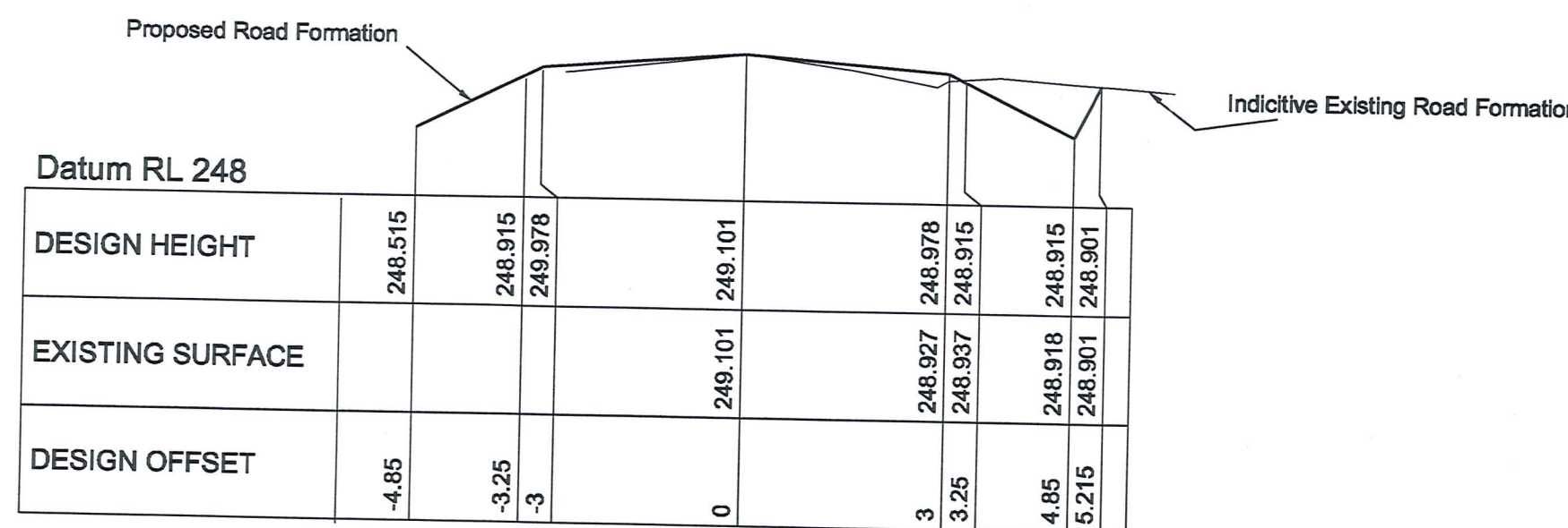
CHAINAGE 300 HORIZONTAL 1:100 VERTICAL 1:50
