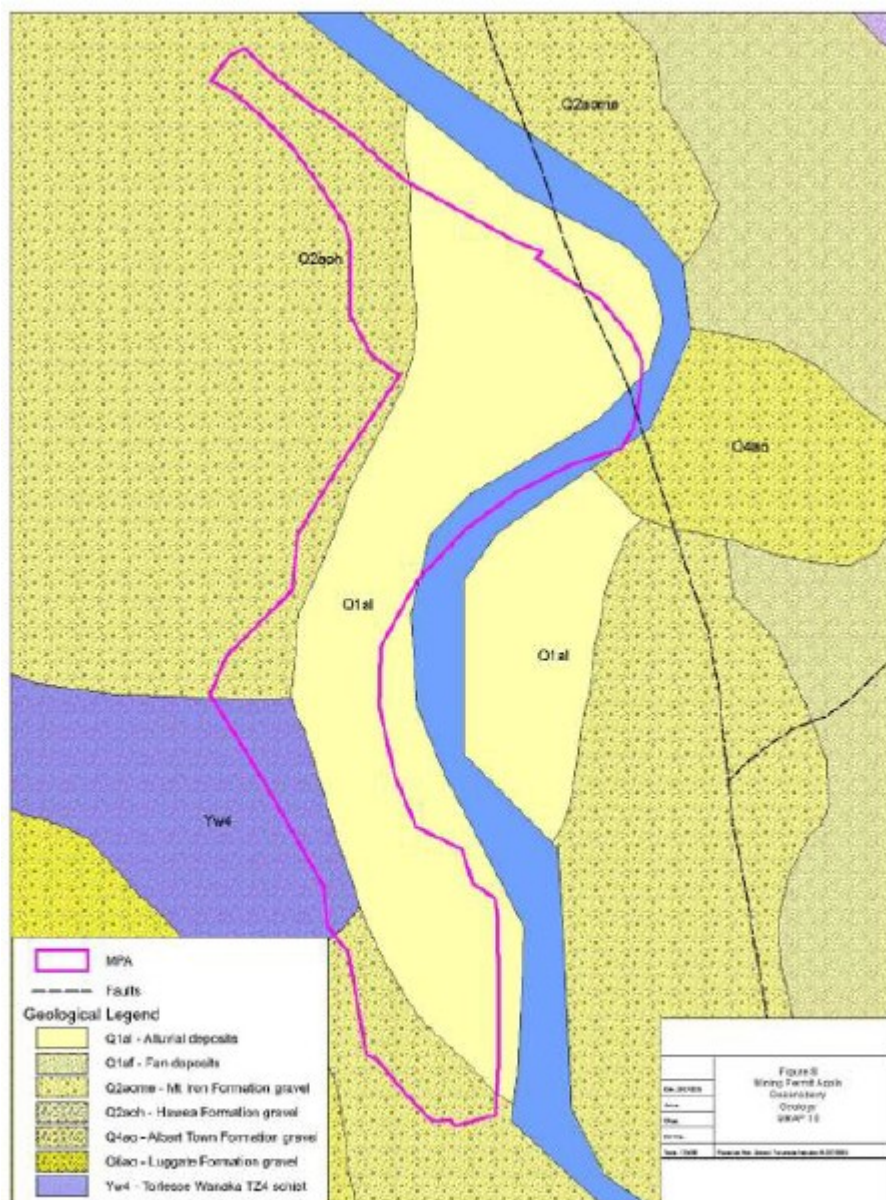
Fig. 5 – Geological Map of Mining Permit Area
