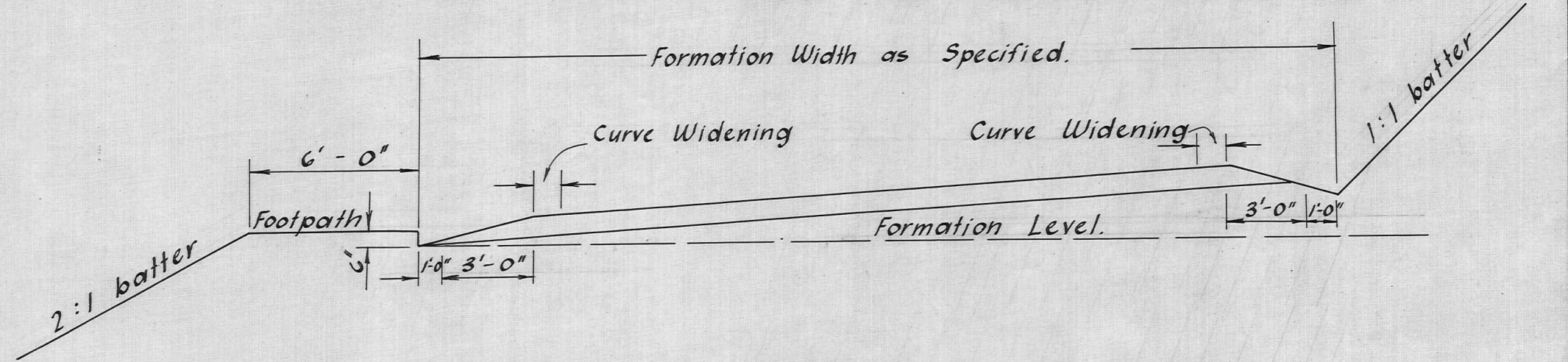
TYPICAL CROSS SECTION ON CURVE Scale: 5 feet to 1 inch.
