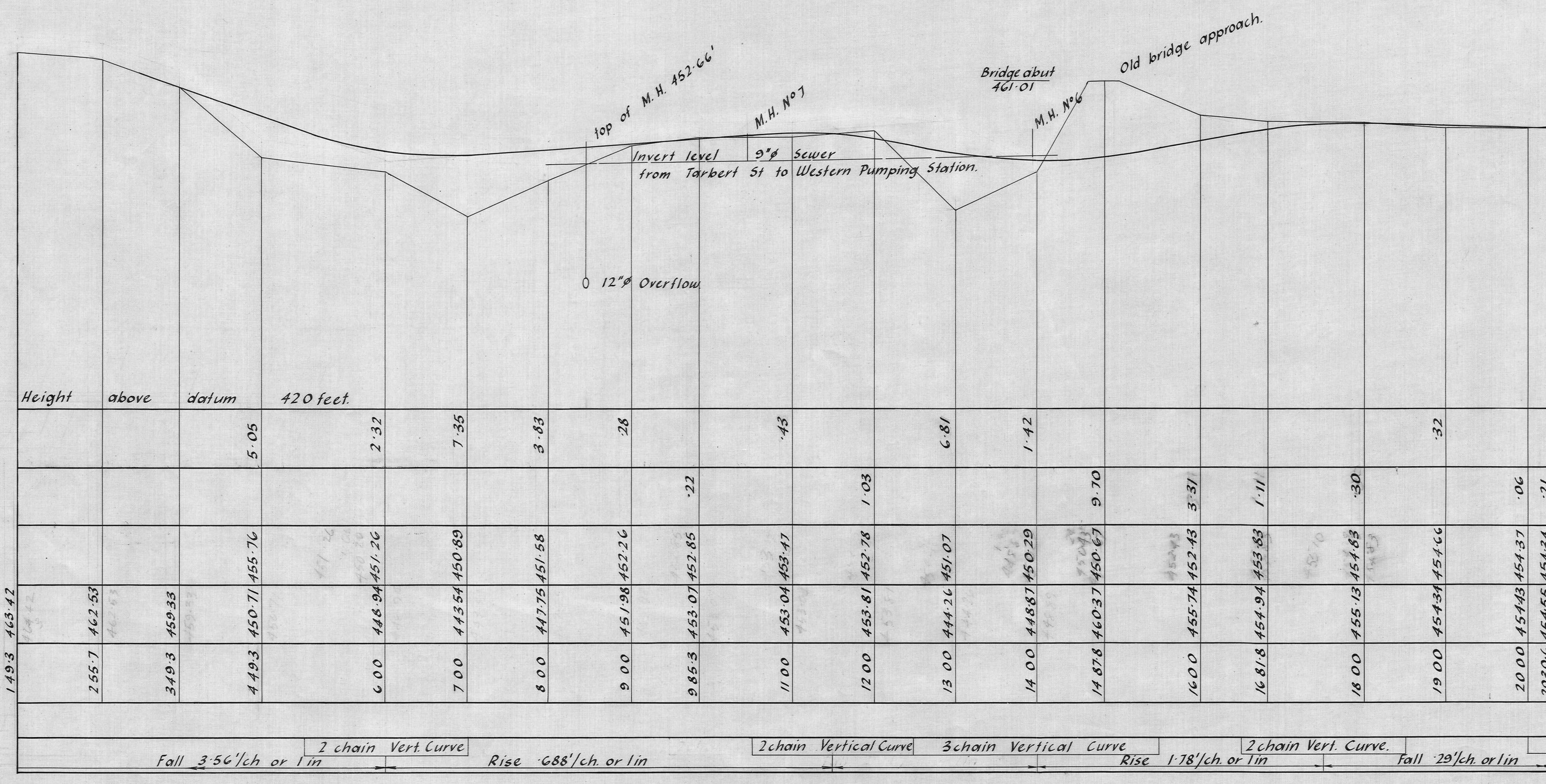
— LONGITUDINAL SECTION — Vertical: 10 feet to 1 inch. Horizontal: 1 chain to 1 inch.
