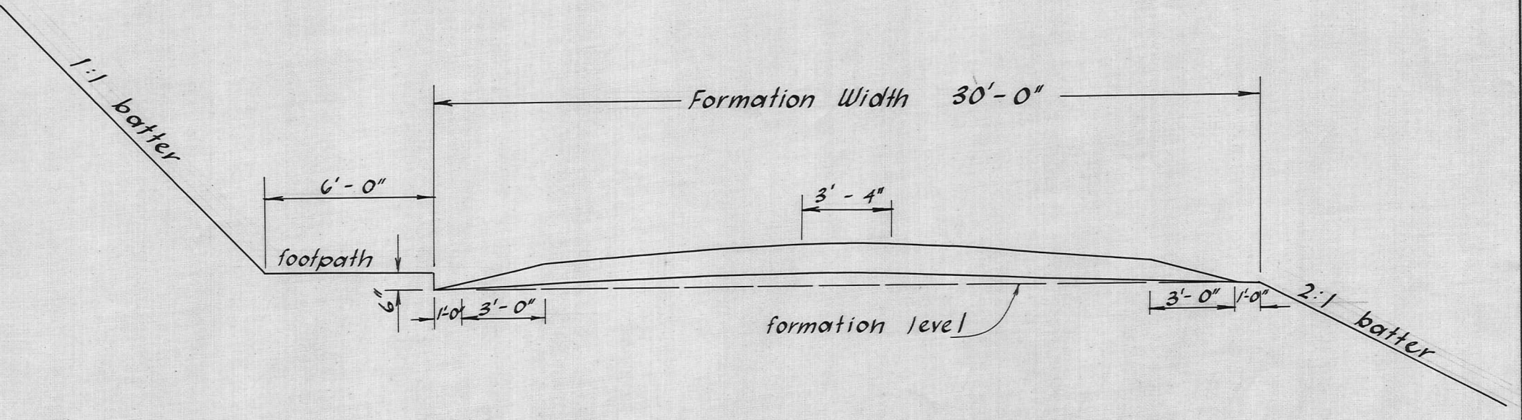
TYPICAL CROSS SEC. ON STRAIGHT
