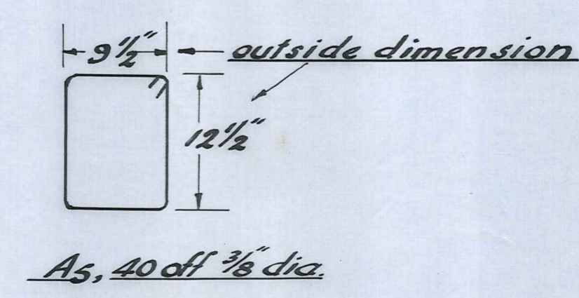
Reinforcing Details Not to Scale
