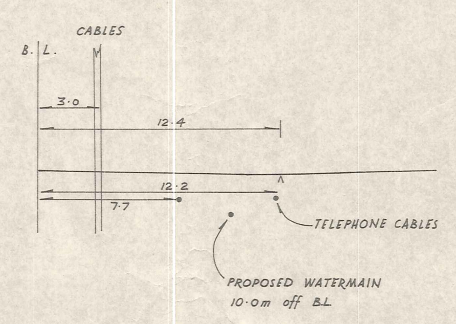
WHITBY TO DUNSTAN SUNDERLAND STREET Scale 1:20
