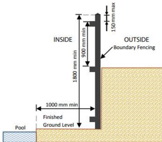
Figure 8: Pool barriers on a property boundary
