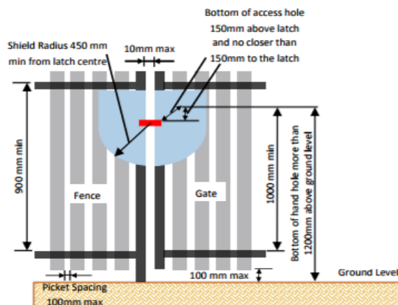
Figure 15: Gate latches for fences less than 1500mm high with a latch shield and access hole
