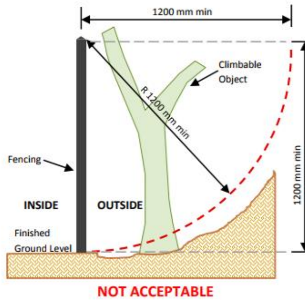
Figure 8: Pool barriers on a property boundary
